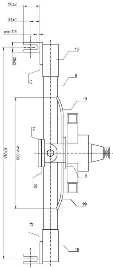
Runner carriers 4 man bob
